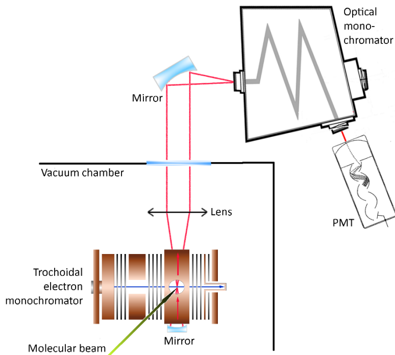
Fig. 1. Experimental apparatus
