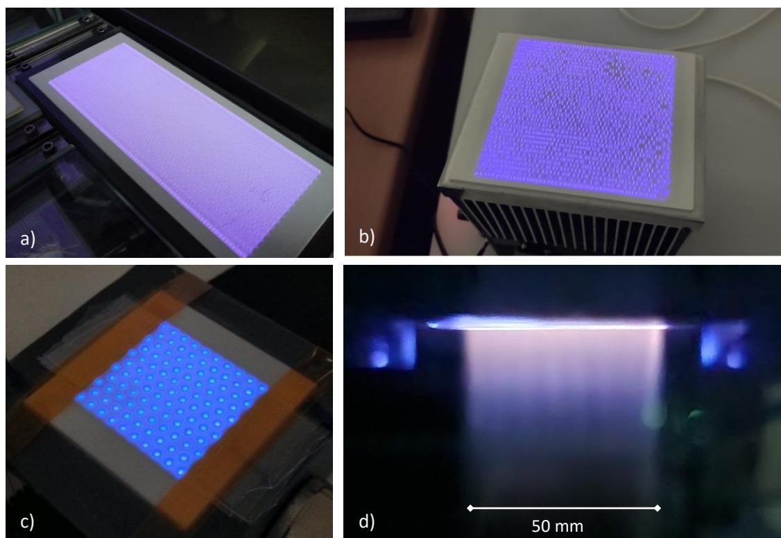
Fig. 1. The photos illustrating plasma generated at atmospheric pressure by DCSBD in ambient air (a), HDCSBD during the heating up period in ambient air (b), MSDBD in flowing air (c), and DCSBD linear APPJ operating into N_2 filled chamber (d).
