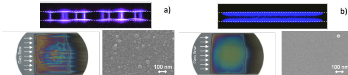
Fig. 3. Comparison of a coating realised with: a) a filamentary discharge and b) a diffuse discharge in N_2 with N_2O and HMDSO for the same discharge power ( 10\text{ W/cm}^3 ).
