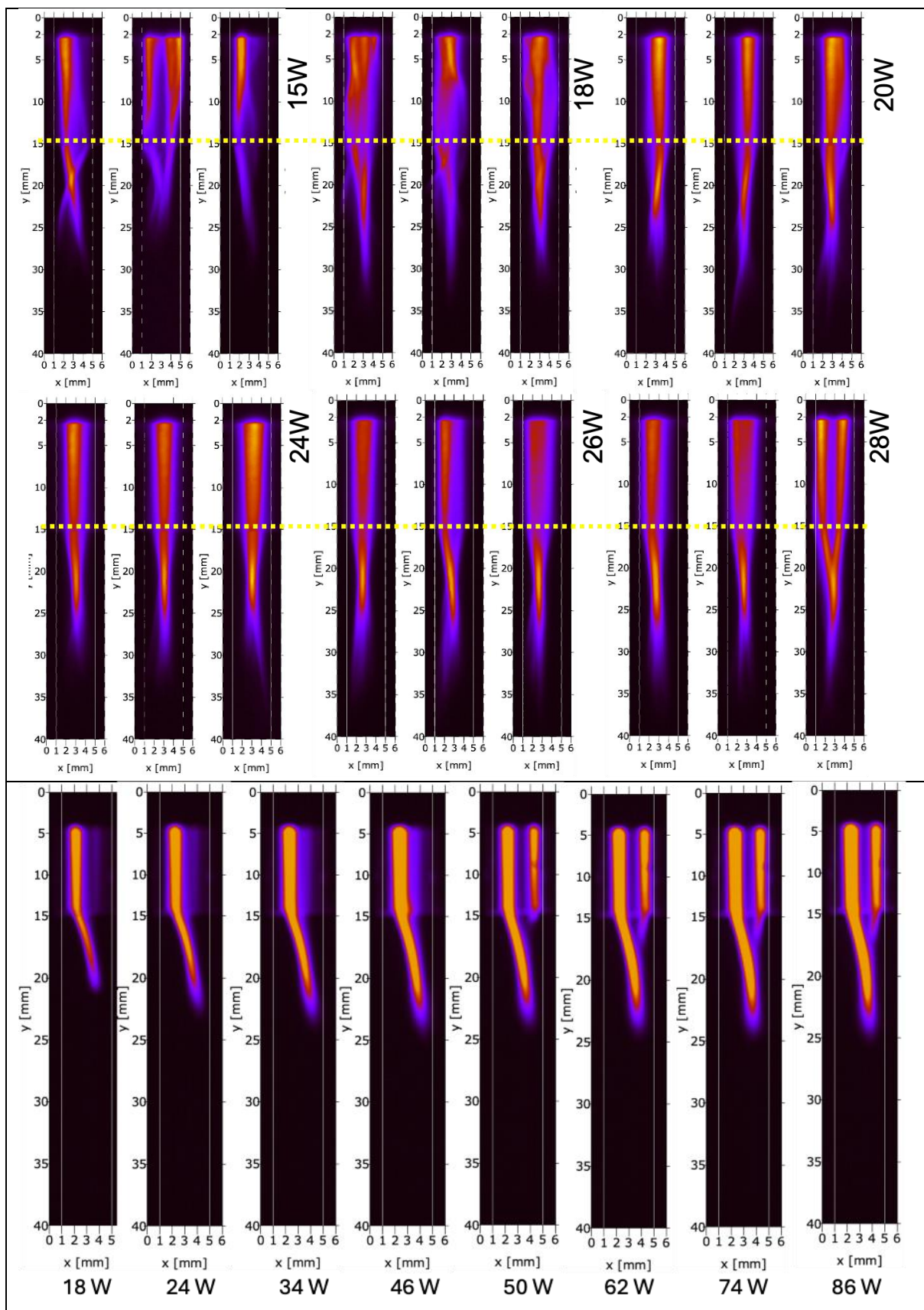
Fig. 5 The CCD images of the 2 slm Ar discharge confined in a 14 mm and 15 mm quartz tubes, respectively, at different input powers in the case of the magnetron and the solid-state generator (lower panel).
