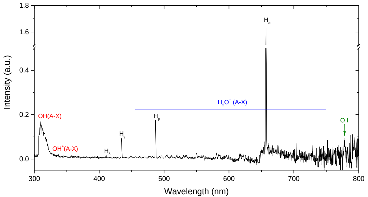
Fig. 2. Emission spectrum of water induced by 50 eV electrons impact.
