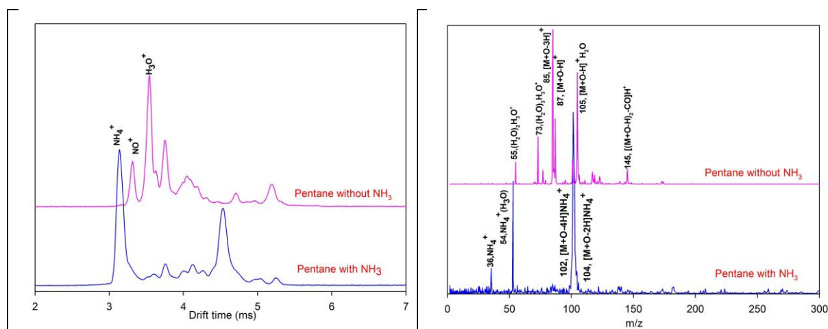
Fig. 2. a) Ion mobility spectra of pentane with and without \text{NH}_3 dopant chamber b) Mass spectra of pentane with and without \text{NH}_3 dopant
