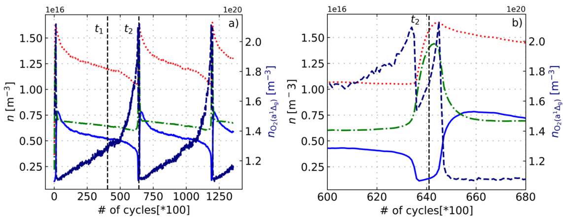
Fig. 3. Time evolution of the density of plasma species: — e^- ..... O_2^+ --- O^- -.- O_2(a^1\Delta_g) . Discharge conditions: 100 Pa pressure, 600 V Voltage amplitude at 13.56 MHz, \gamma = 0.0042 .
