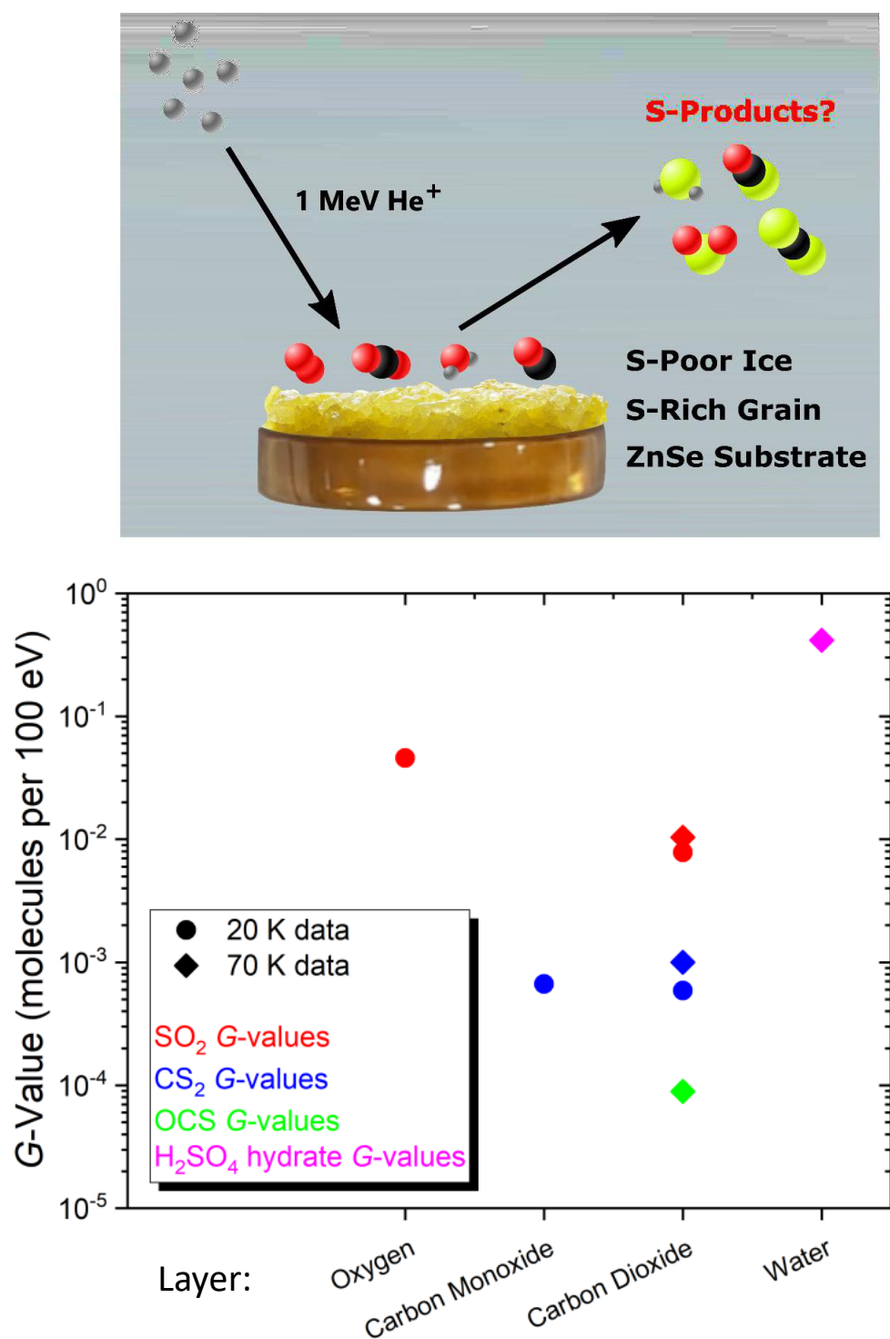
Fig. 2. Obtained G-values (number of produced molecules per 100 eV deposited energy) for the sulphur-bearing products observed as a result of irradiating different ices on top of allotropic sulphur using 1 MeV He + ions. Note that circles represent data points acquired at 20 K, while diamonds represent those acquired at 70 K.
