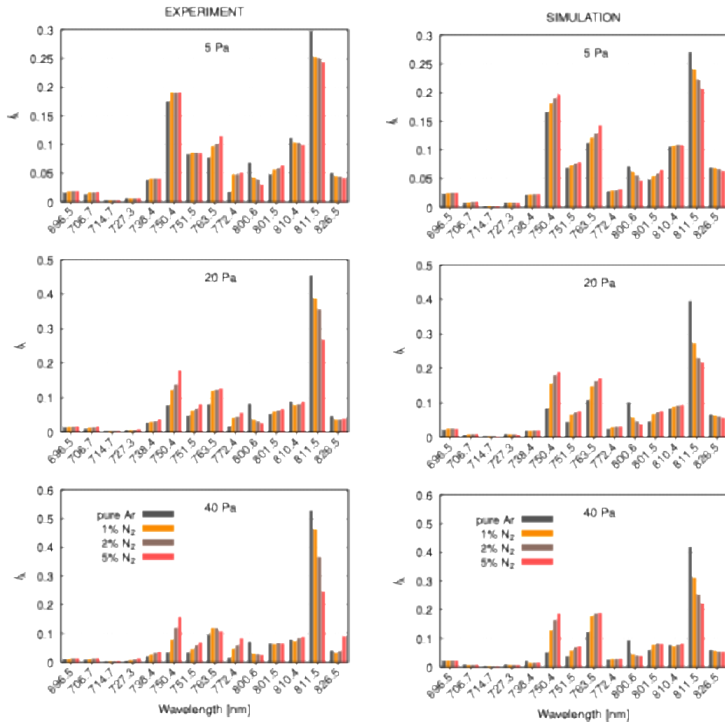
Fig. 4. Measured (left) and computed (right) relative intensities of Ar 2p \rightarrow 1s spectral lines at the center of the discharge, for various pressures and nitrogen contents.
