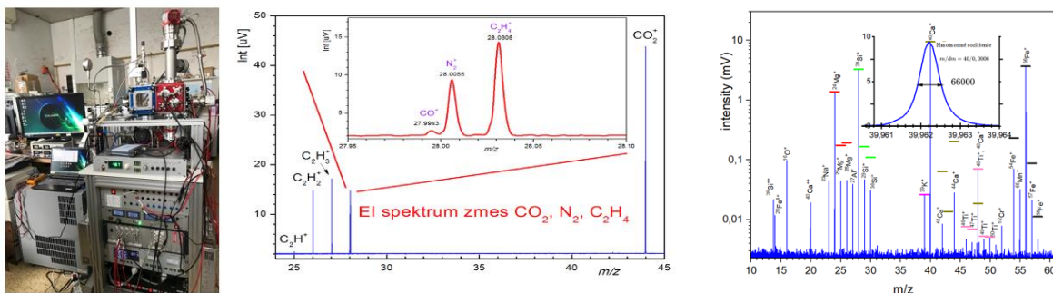
Fig. 1. HANKA – laboratory prototype, the data: EI source [3] and plasma source -Martian meteorite
