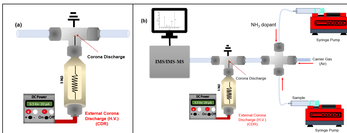
Fig. 1. a) Schematic view of external corona discharge reactor, b) experimental setup for ionization of alkanes with \text{NH}_3 dopant.
