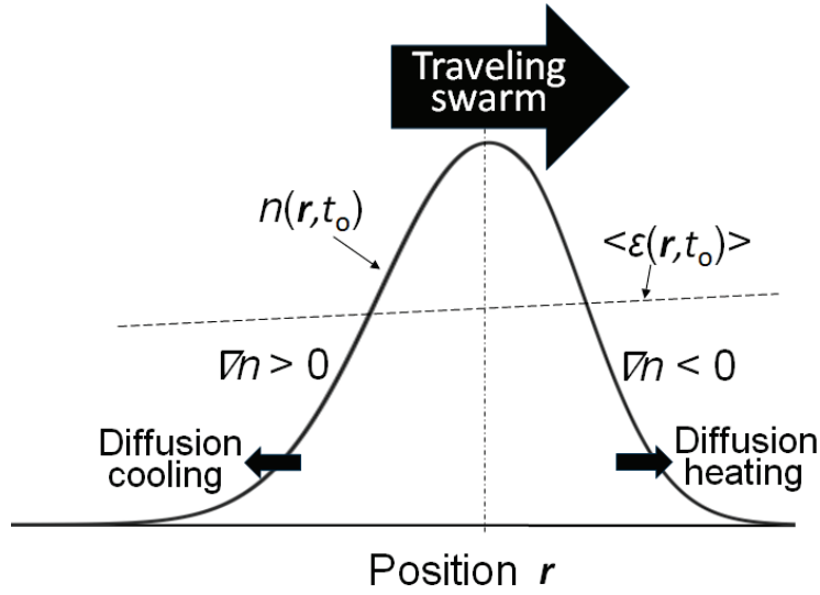
Figure 2. An isolated traveling swarm of charged particles with number density n(\mathbf{r}, t_0) at time t_0 in gases in an external field. \langle \epsilon(\mathbf{r}, t_0) \rangle is the local mean energy.
