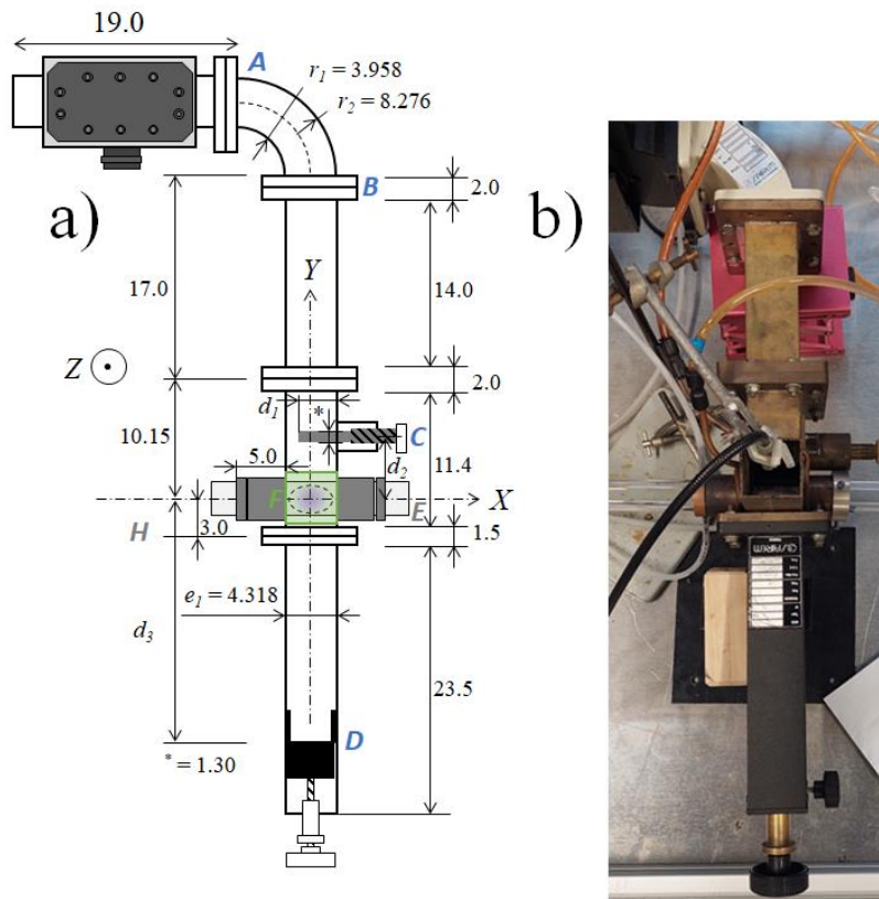
Fig. 1. a) Schematic of the microwave delivery system used for the microwave-discharge interaction model. Distances are in cm. Letters are used to locate the different parts of the system. The copper window enables the viewing of the plasma from the bottom and the top is perpendicular to the view plane and depicted in green. b) Picture of the experimental setup showing the WR-340 waveguide, the movable stub, the short-circuit piston, and the reactor tube. The height of the waveguide is 8.636 cm.
